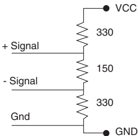
SCSI termination
