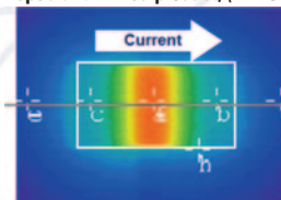
Temperature distribution of a special trimmed product, (TLR Series)
