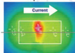
Temperature distribution of a line-trimmed product
