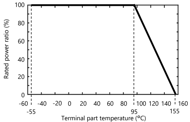
Fig. 6 WK73R series and the derating curve based on the terminal part temperature
